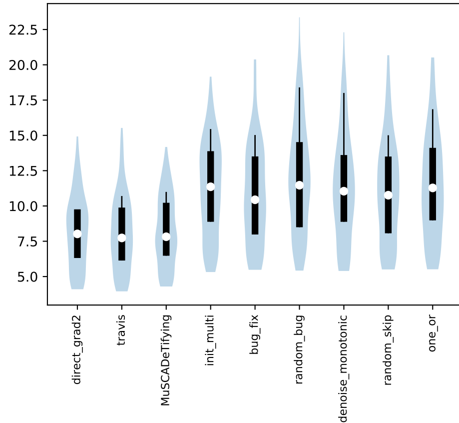
init time
